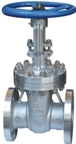
Cast Stainless Steel Gate valve ZZ-002
